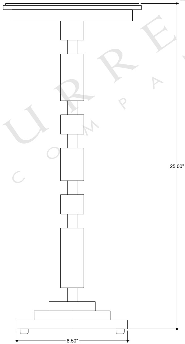
FRONT VIEW
